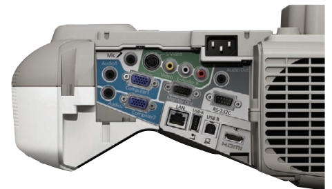
EB-485W interface
